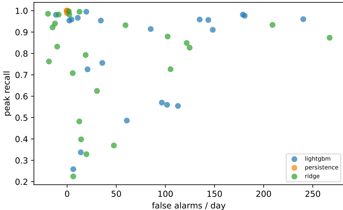
Peak recall vs false alarms (q95, dev)
