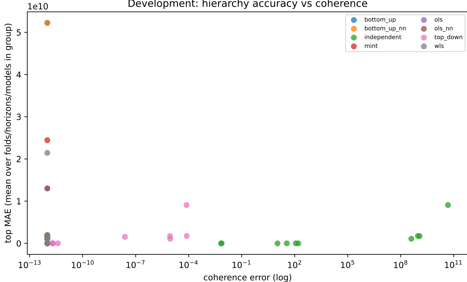
Development: hierarchy accuracy vs coherence
