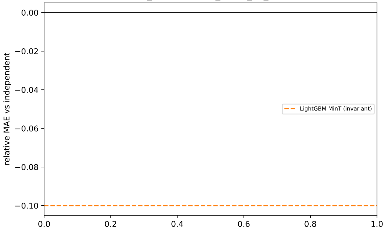
cpu_reconciliation_effect_by_seed
