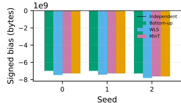
DLinear memory peak bias (q95)
