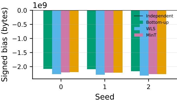
DLinear memory peak bias (q90)
