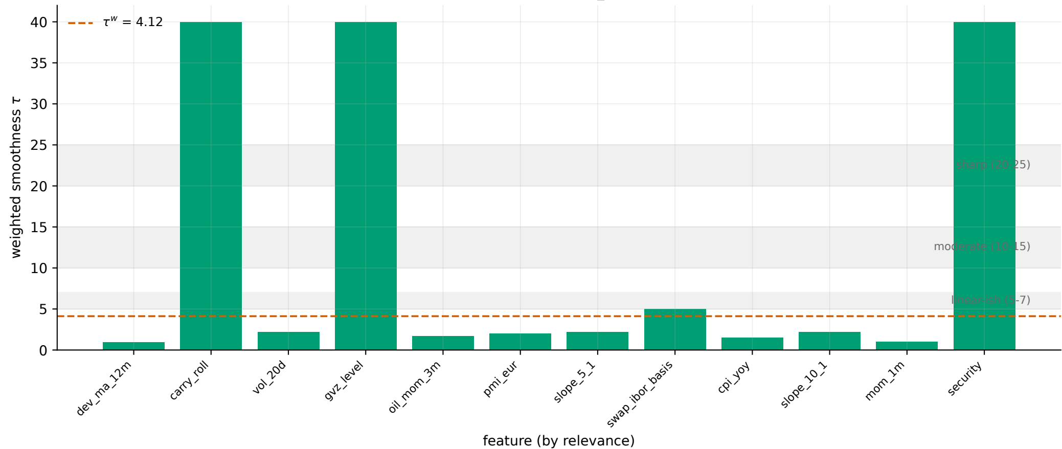
HTBoost per-feature smoothness \tau — pooled HTBoost-L2, H=21, ZIRP_early fold (representative fit: 31 trees, depth 3, \tau^w=4.12 )
