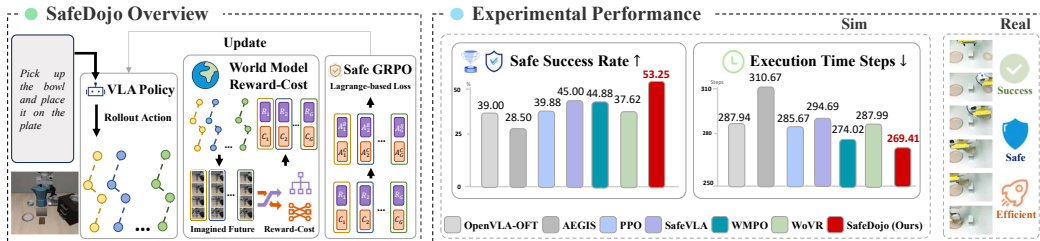
Figure 1: Overview of SafeDojo. SafeDojo enhances VLA policies with world-model-based reward-cost evaluation and safe GRPO, boosting safe success and efficiency in simulation and real-world scenarios. The performance panels compare against all baselines; complete comparisons are reported in Tables 1 and 2.
