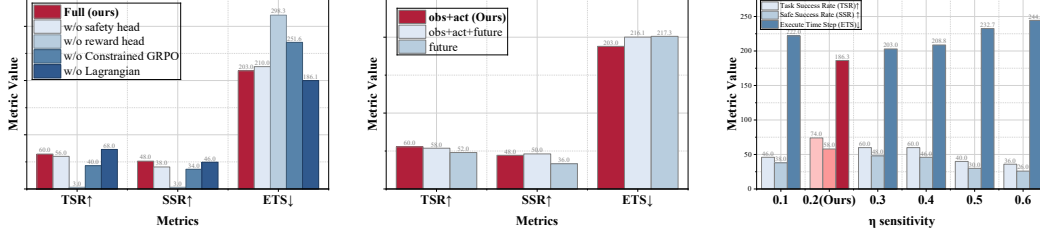
Figure 4: Ablation studies on SafeLIBERO Level I Spatial Task 0. Left: component ablation by removing each design choice independently. Center: input-source ablation comparing three configurations for reward–cost estimation. Right: sensitivity analysis of the initial safety cost weight \eta .
