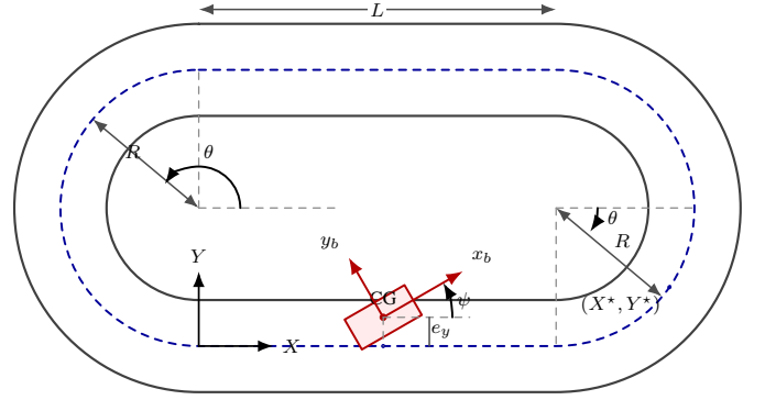
Fig. 2: Geometry of the stadium path and vehicle pose.
