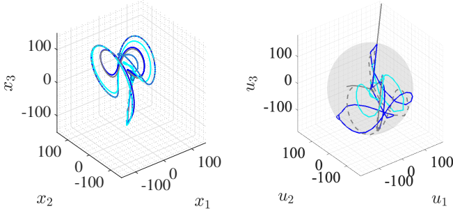
(a) State trajectories (3D-view). (b) Control input loci (3D-view).
