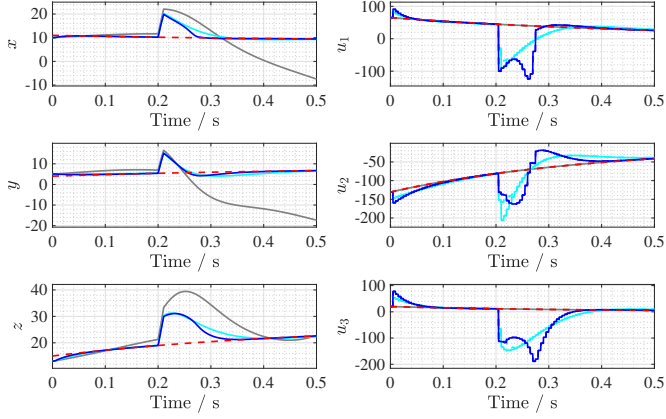
Fig. 2. Numerical validation results of (C 1 ) [—], (C 2 ) [—], (C 3 ) [—], and desired trajectory x_d [—].
