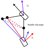
Effect of reversal-phase control (high speed)
