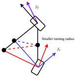
Effect of reversal-phase control (low speed)
