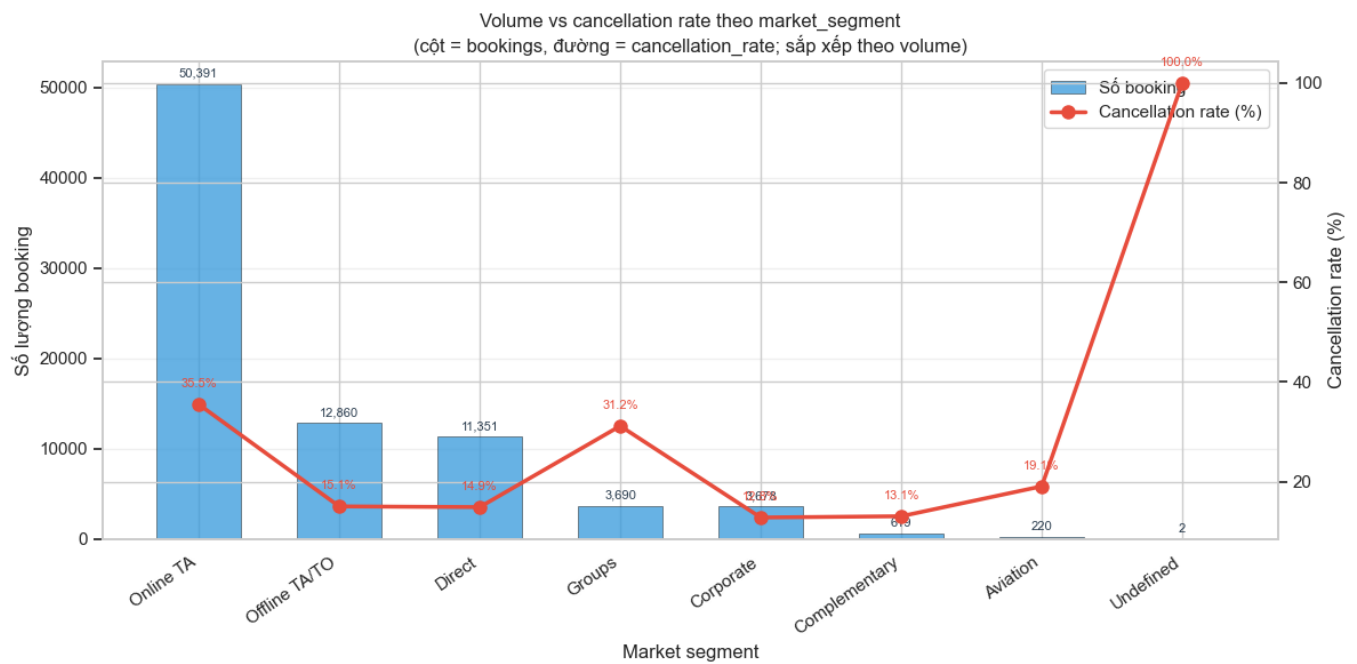
Biểu đồ 9: Dual-axis — Volume vs cancellation rate theo market_segment
