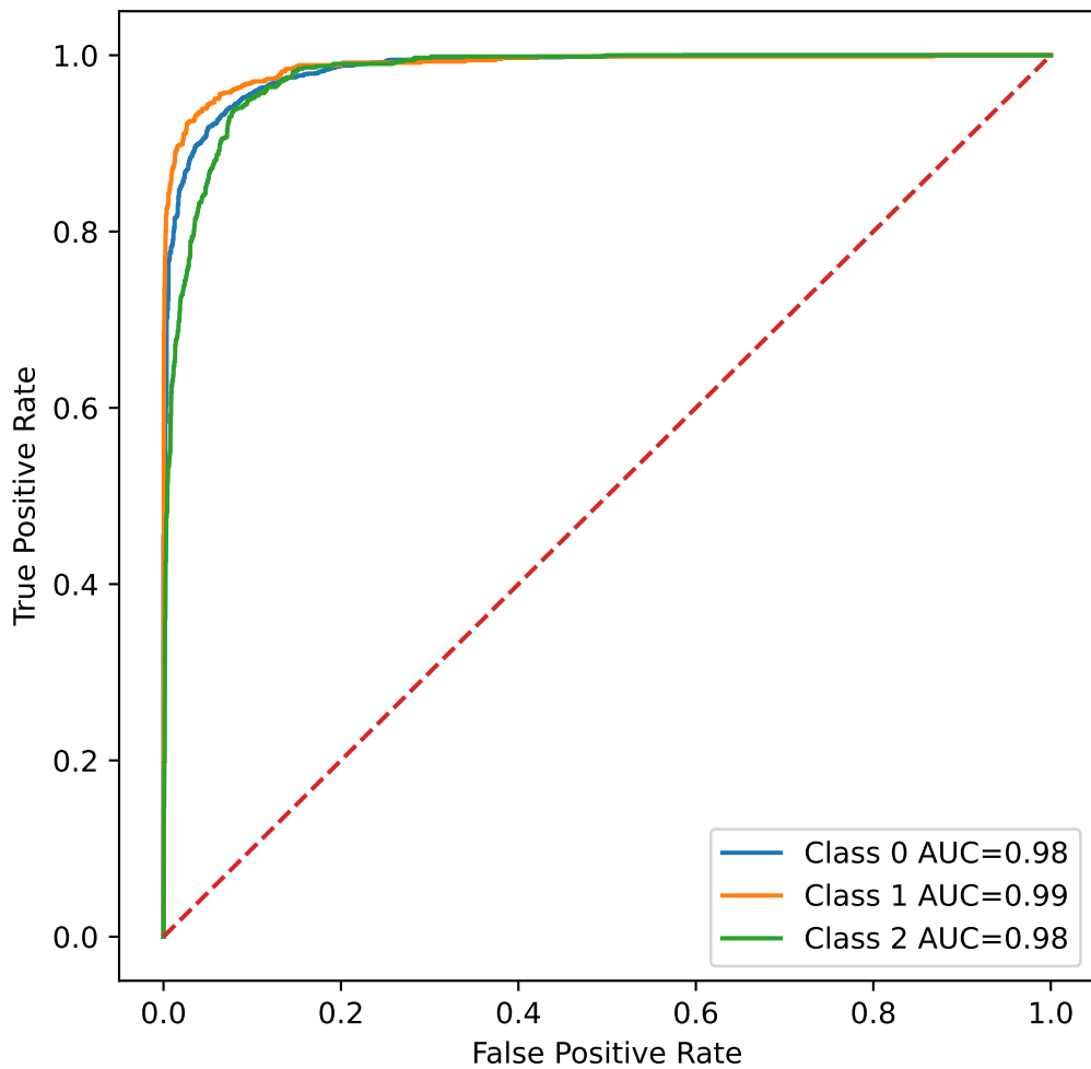
ROC Curve - CNN
