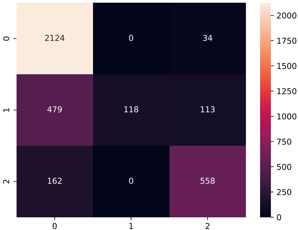
EfficientNetB0 Confusion Matrix
