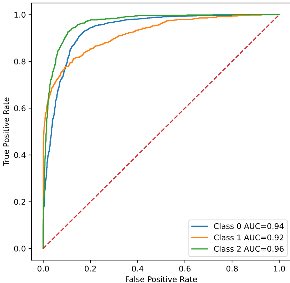
ROC Curve - EfficientNetB0
