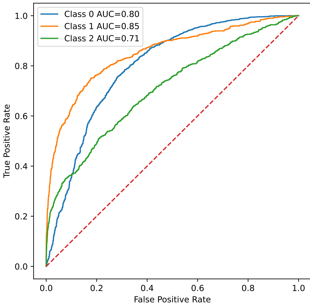
ROC Curve - MobileNetV2
