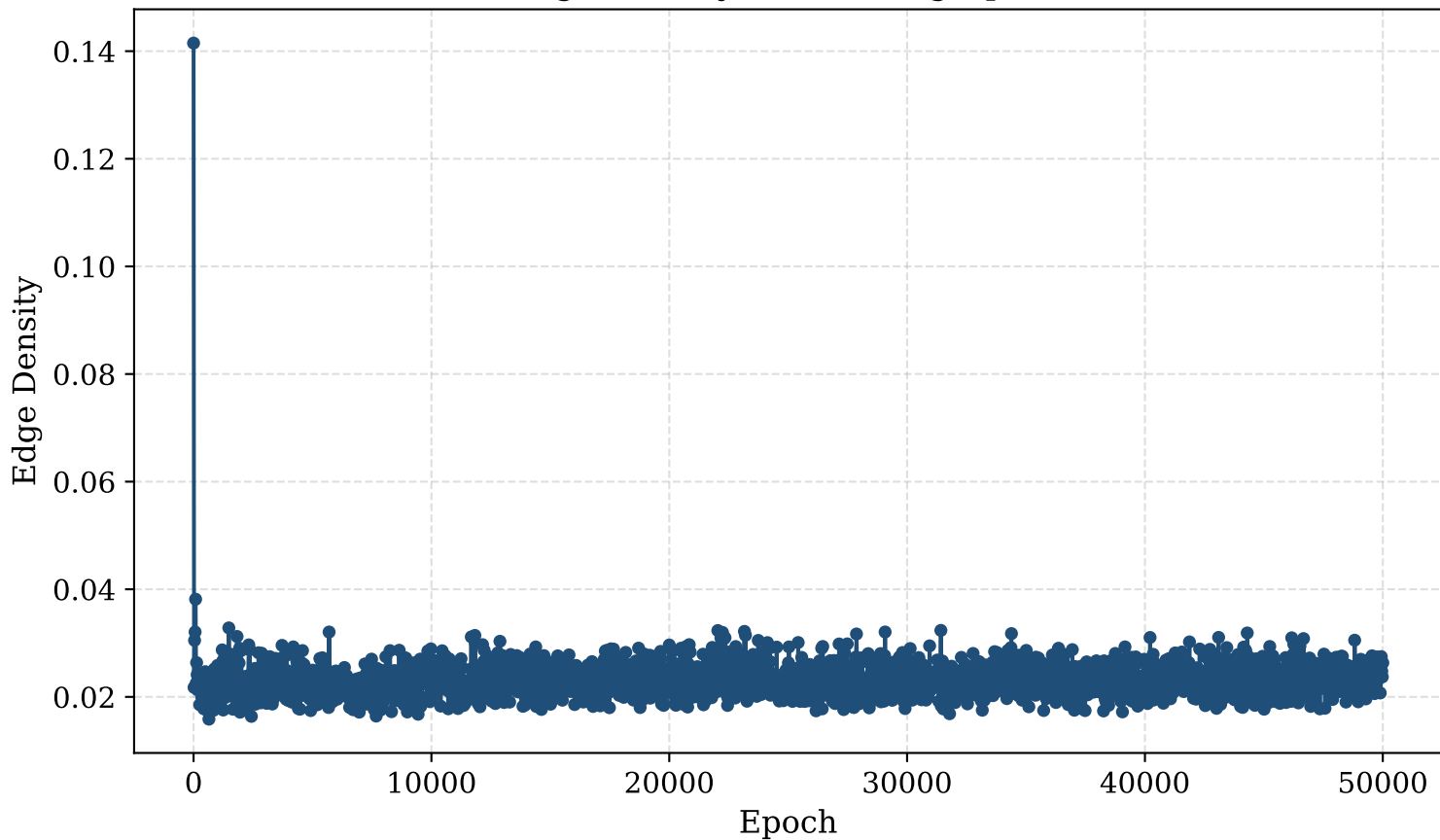
Edge Density vs. Training Epoch
