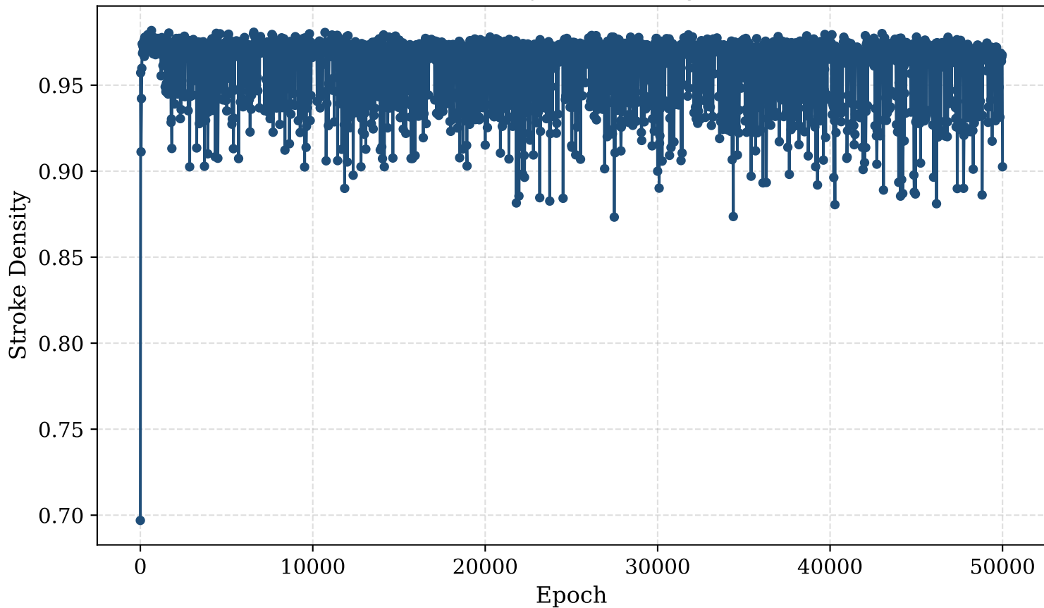
Stroke Density vs. Training Epoch
