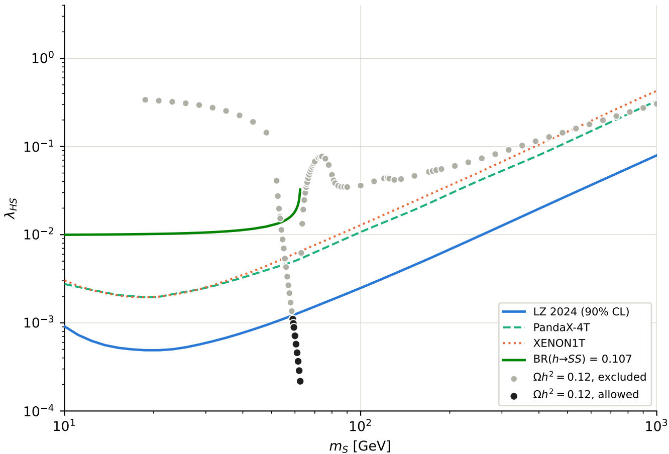
Points with \Omega h^2 = 0.12 (SPHeno \rightarrow micrOMEGAs)
