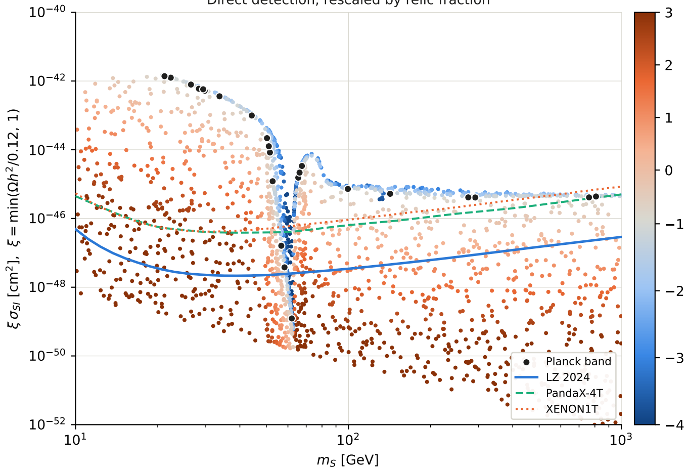
Direct detection, rescaled by relic fraction
