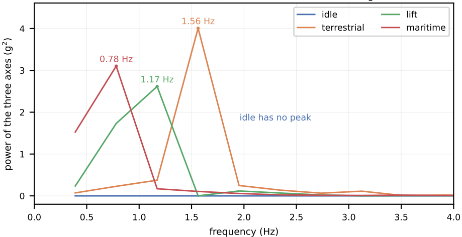
One 2 s window of session s1, the three axes added, FFT length 128
