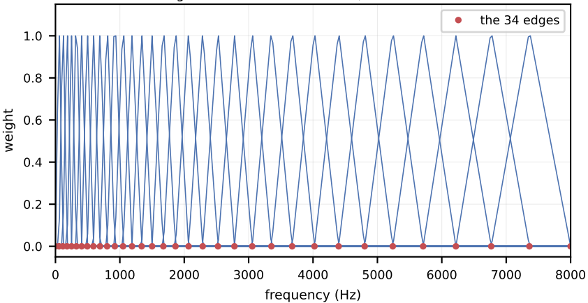
32 triangular filters of the Mel scale, 257 bins of 31.25 Hz
