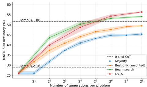
Llama 3.2 1B on MATH-500, with an 8B process reward model
