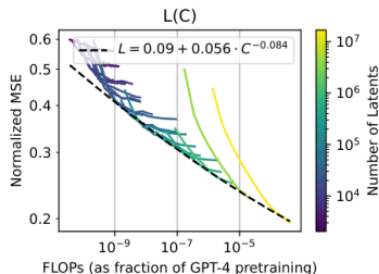
Reconstruction error against SAE training compute.
