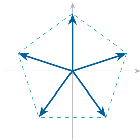
5 sparse features in 2 dimensions
