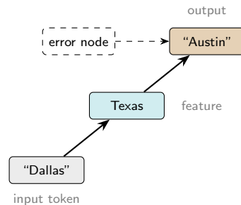
Schematic of a two-hop attribution graph.
