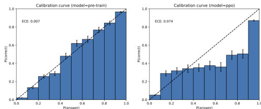
GPT-4 on an MMLU subset. Left: after pre-training, ECE 0.007. Right: after PPO post-training, ECE 0.074.
