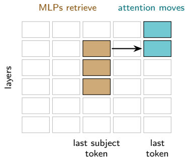
Schematic of the causal-tracing finding.
