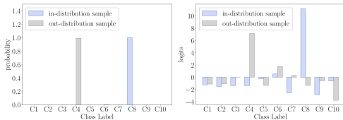
(a) softmax scores 1.0 vs. 0.99
