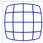
barrel, k_1 = -0.12
