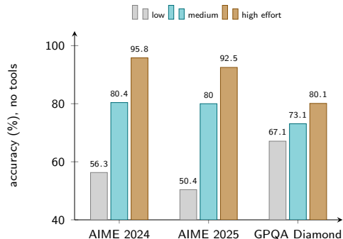
gpt-oss-120b at three reasoning-effort levels
