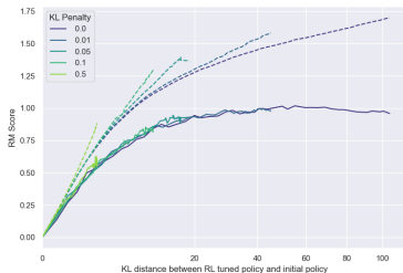
Gold score against KL, for five KL penalties.
