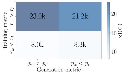
DPO training pairs: reward ranking (rows) against likelihood ranking (columns).
