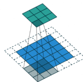
padding = 1, stride = 2
