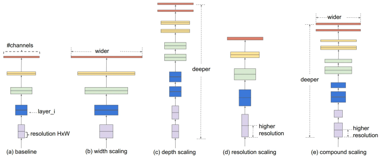
Figure 4: EfficientNet Scaling.
