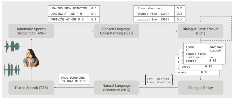
Figure 2: Architecture of dialogue-state system for task-oriented dialogue (Williams et al., 2016)
