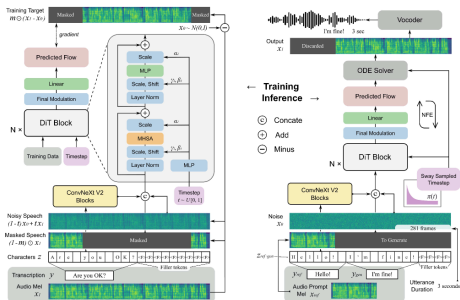
F5-TTS training (left) and inference (right). Chen et al., "F5-TTS: A Fairytaler that Fakes Fluent and Faithful Speech with Flow Matching," arXiv:2410.06885 , Figure 1.
