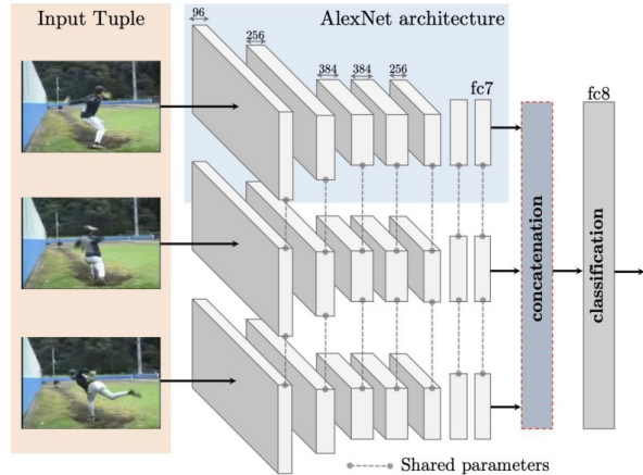
Triplet Siamese network for sequence verification
