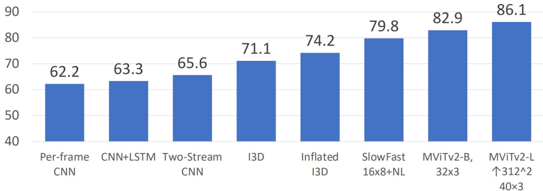
Top-1 Accuracy on Kinetics-400
