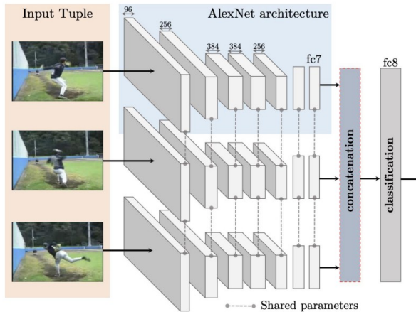
Triplet Siamese network for sequence verification
