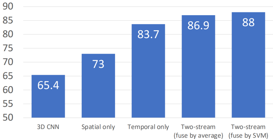
Accuracy on UCF-101
