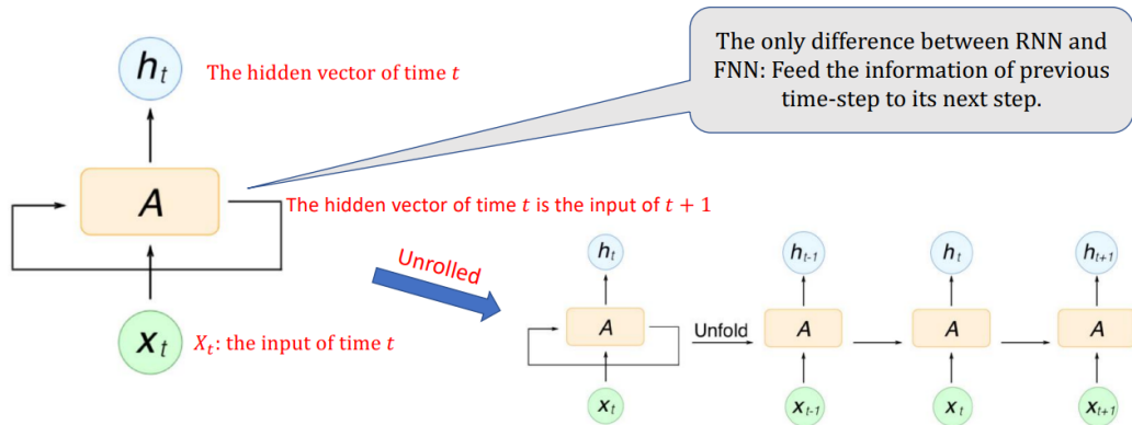
Recurrent Neural Network (RNN) sample architecture.
