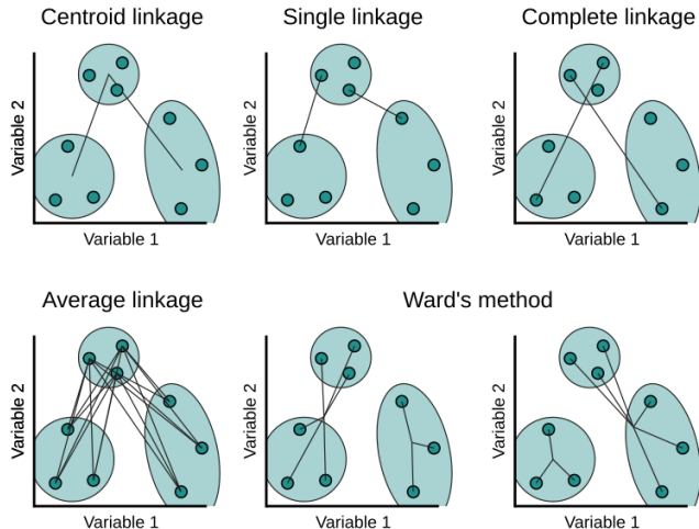
Figure 20: Linkage methods.
