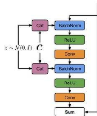
BigGAN '18 355 million parameters, trained on 512 TPU cores
