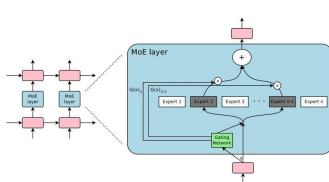
Sparsely gated mixture of experts '17 130 billion parameters, trained on 128 GPUs
