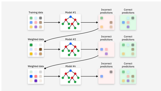
Figure 6: Boosting Example
