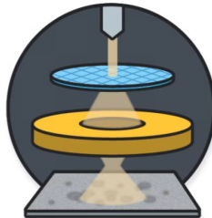
Cryoelectron microscopy
