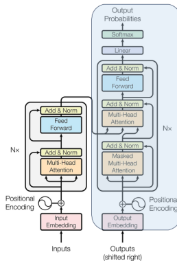
Diagram: Vaswani et al., NeurIPS 2017,
