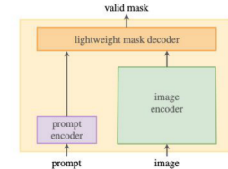
(b) Model: Segment Anything Model (SAM)
