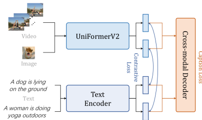
(b) Multimodal Video Encoder
