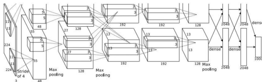
Krizhevsky et al. 2012. 8-layer “AlexNet”.
