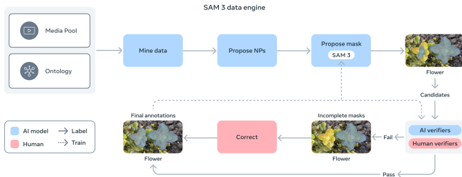
SAM 3 data-engine loop from Meta blog post.
