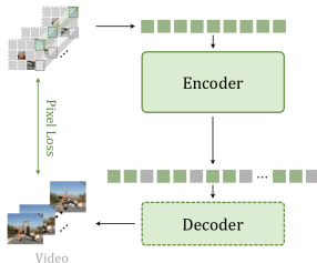
(a) Masked Video Encoder
