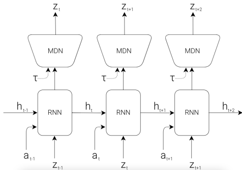
MDN-RNN architecture.
