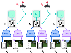
(a) World Model Learning
