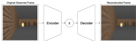
VAE diagram.
