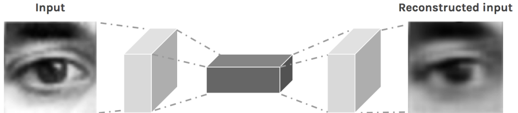
Sample Autoencoder
