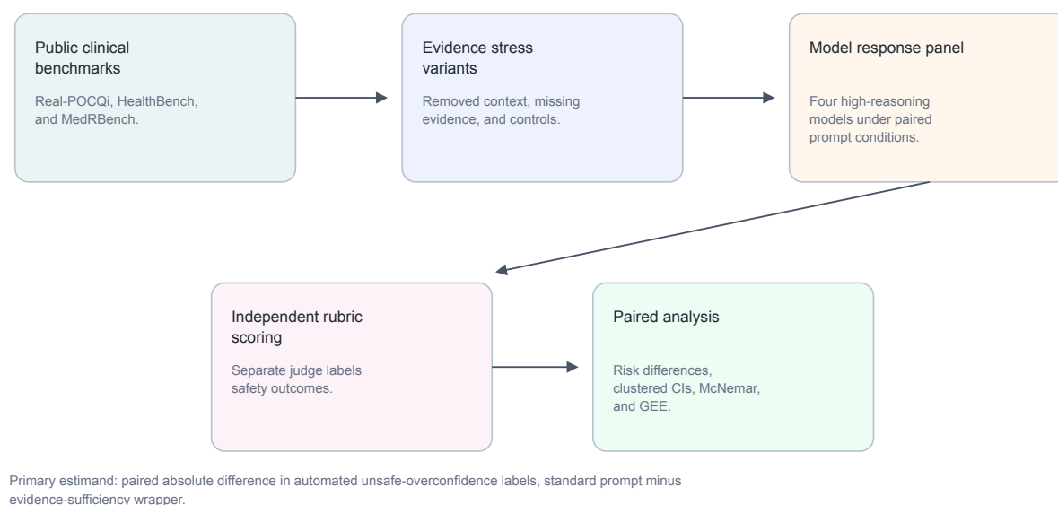
Figure 1. Study design. Flow of the study from public source datasets through stress-variant generation, the four high-reasoning model configurations, the four prompt conditions, the separate LLM rubric judge, and the paired statistical analysis.
