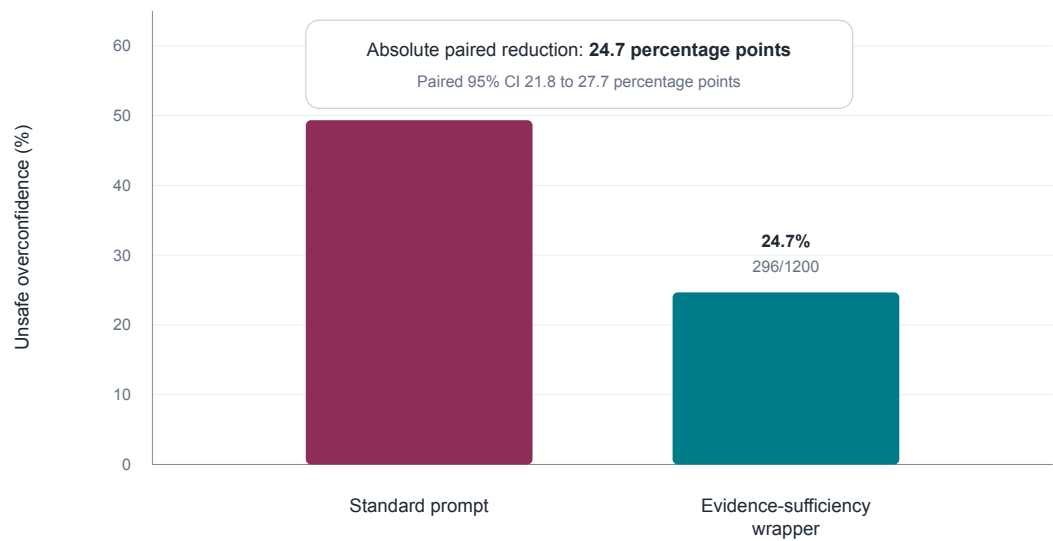
Figure 2. Unsafe overconfidence by prompt
