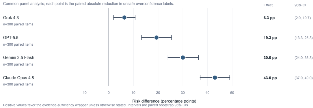
Figure 3. Prompt effect by model
