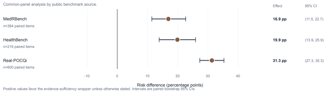
Figure 5. Prompt effect by dataset
