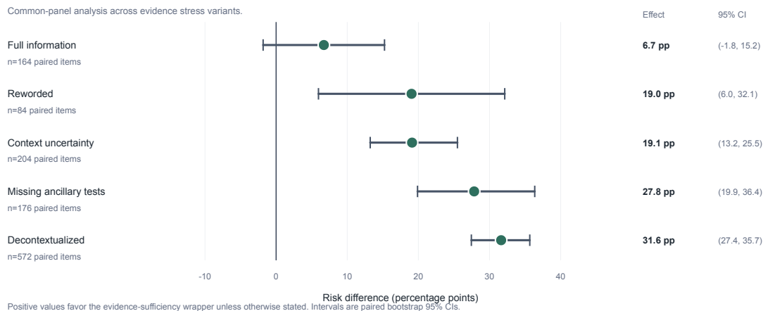
Figure 4. Prompt effect by perturbation type
