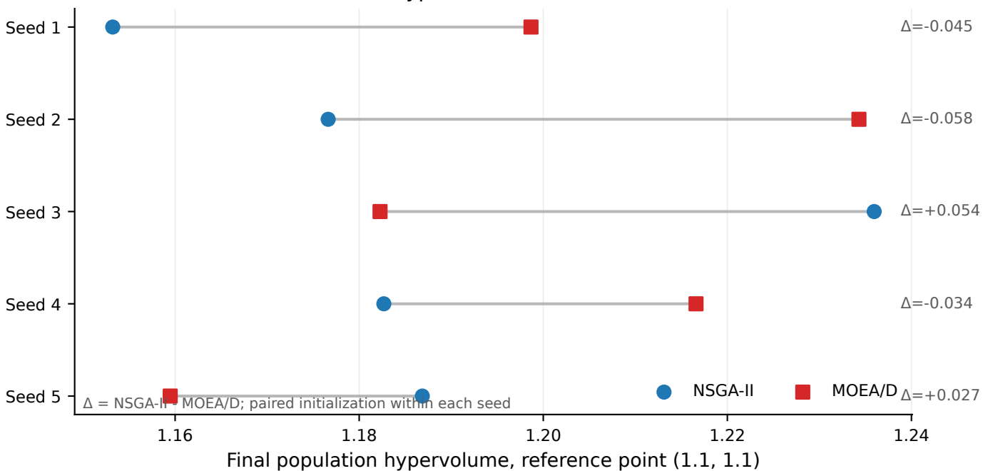
Paired final hypervolume across five seeds
