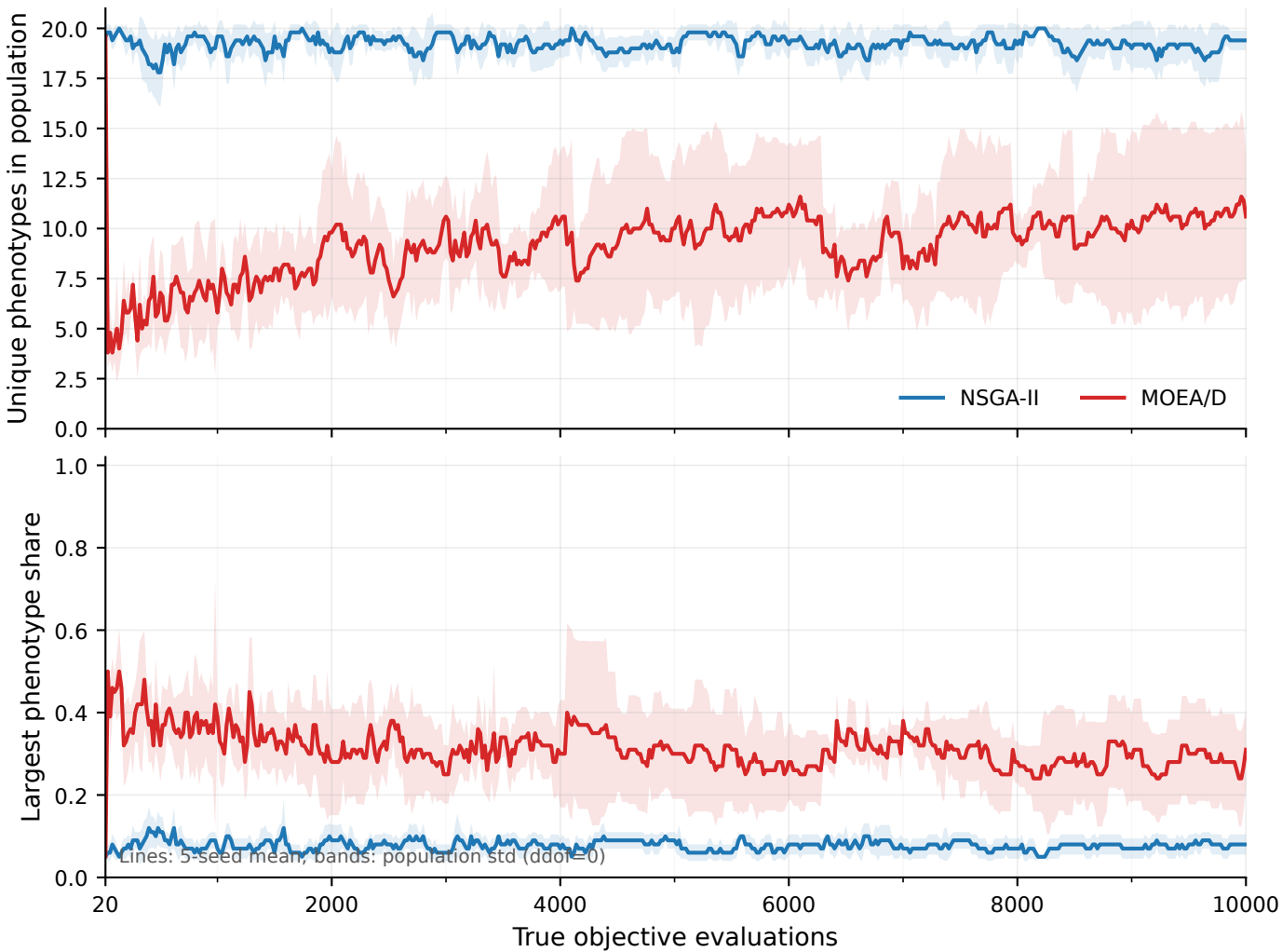
Phenotype diversity during search
