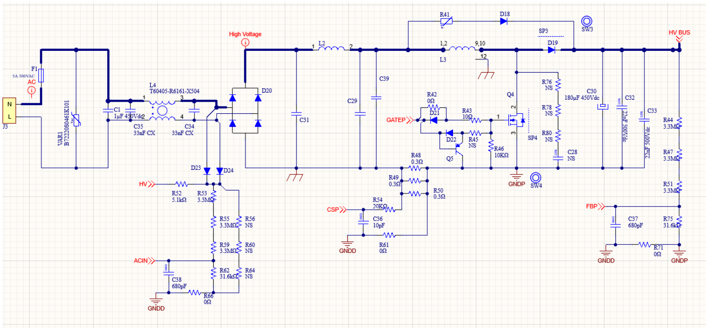
Figure 7: Altium design of the input front end: connectors, EMI filter, bridge rectifier, and boost PFC.
