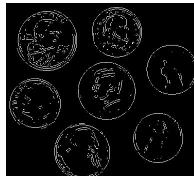
Prewitt - b.2
