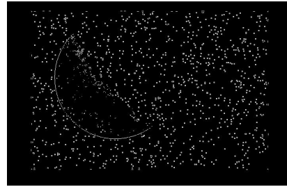
Prewitt - b.2
