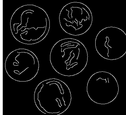
Canny sigma=3.0
