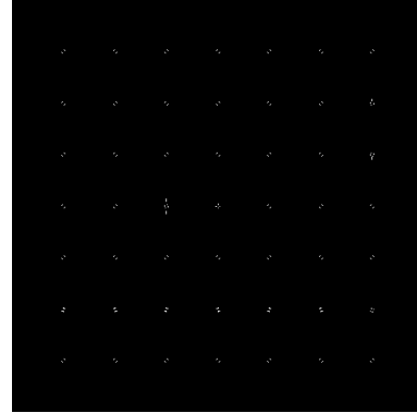
Prewitt - b.2
