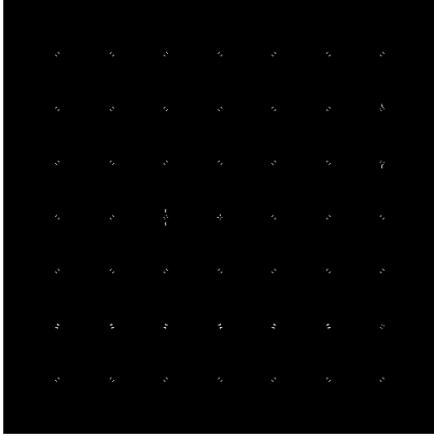
Prewitt - b.1
