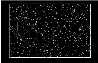
Prewitt - b.1
