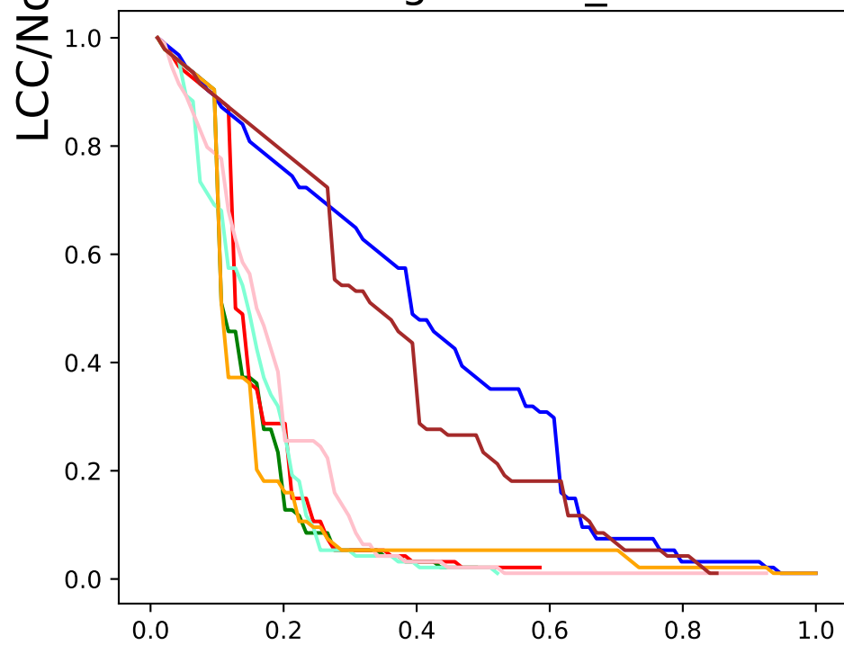
homogeneous_100
