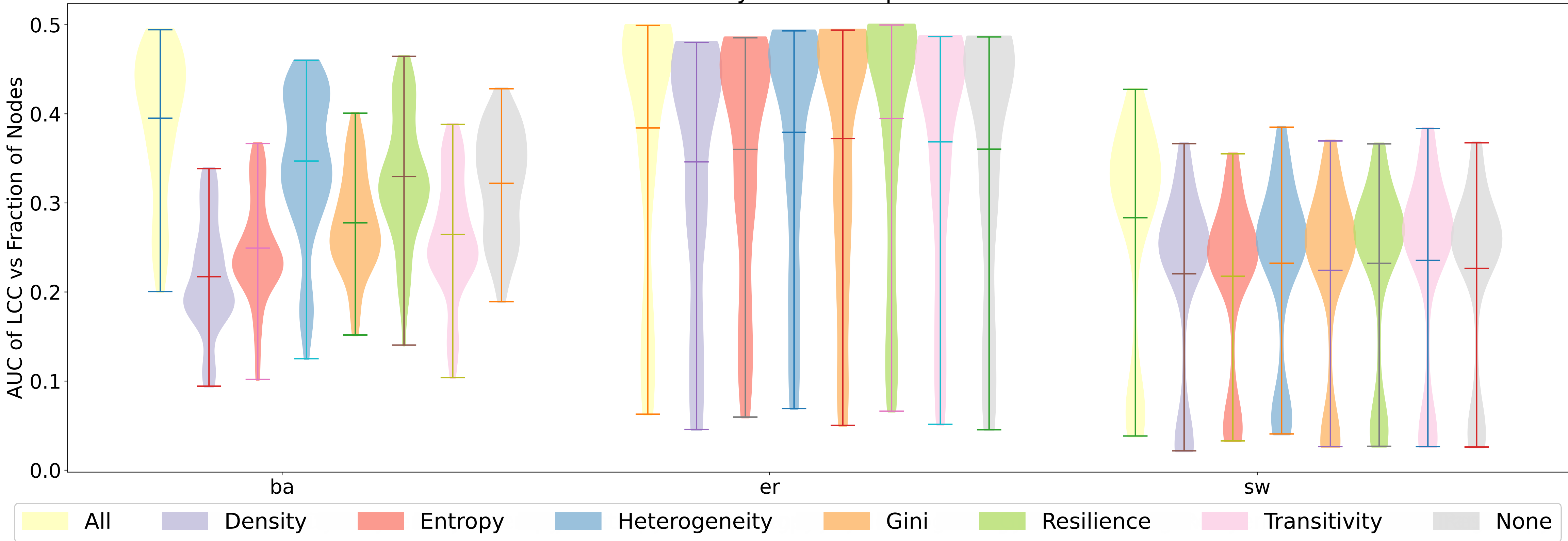
Synthetic Graph
