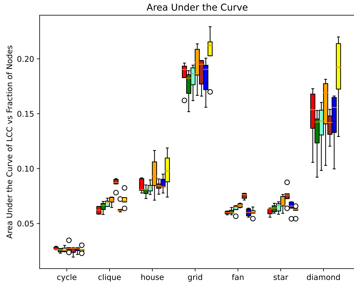
Synthetic Graph with Motifs: Comparison with Different Global Properties (Mix). Tree Base Graph
