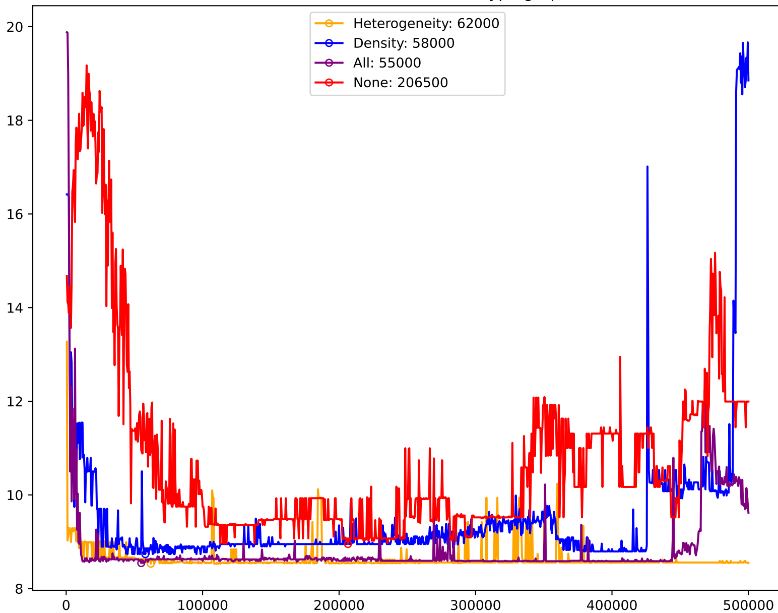
AUC of LCC vs Nodes Plot BA type graph
