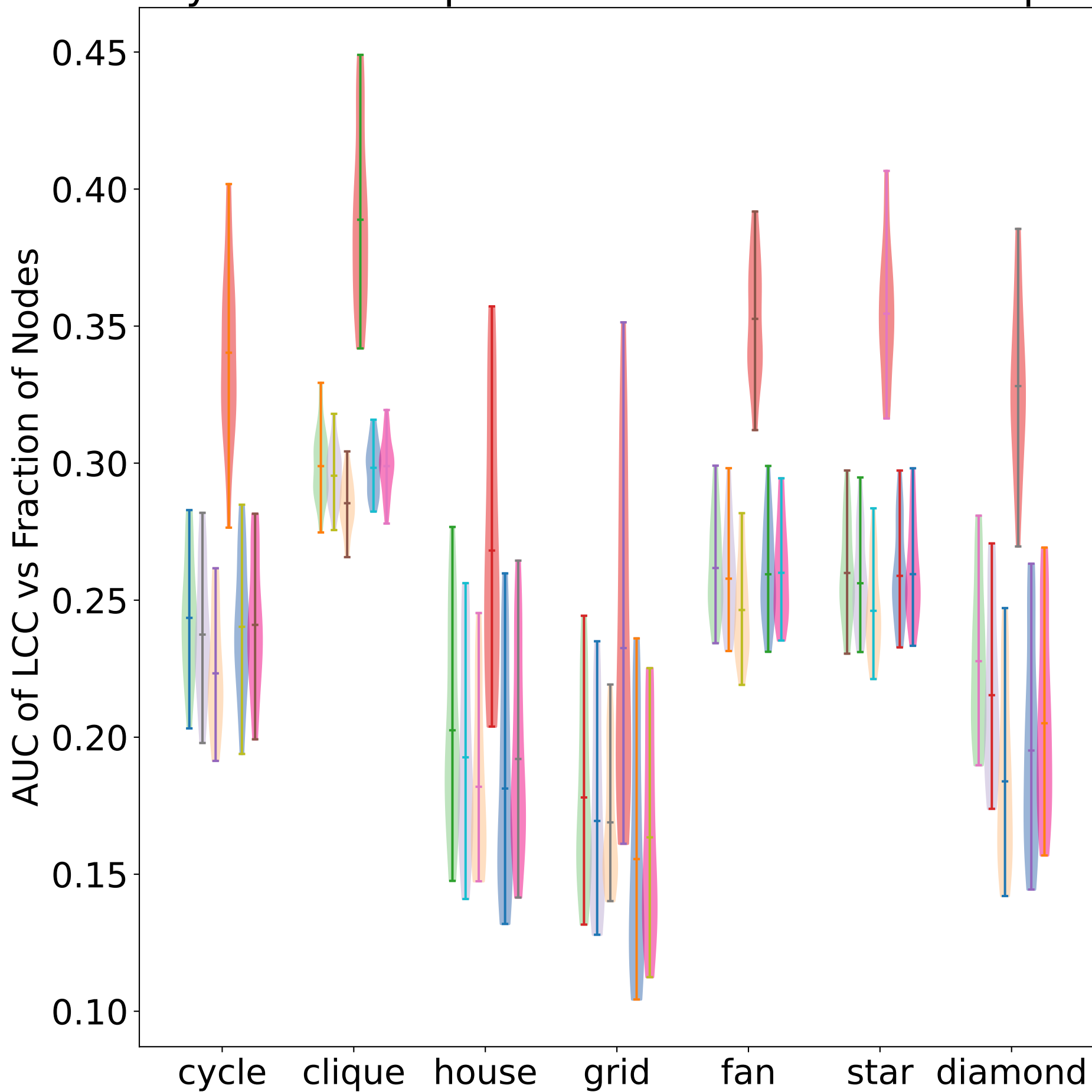
Synthetic Graph with Motifs: BA Base Graph
