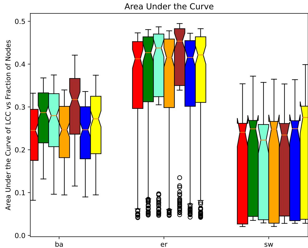
Synthetic Graph: Comparison with Different Global Properties (MIX). Degree evaluation
