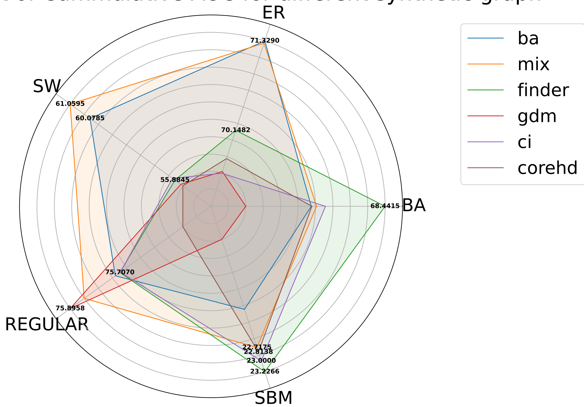
Radar Chart of Cumulative AUC for different synthetic graph
