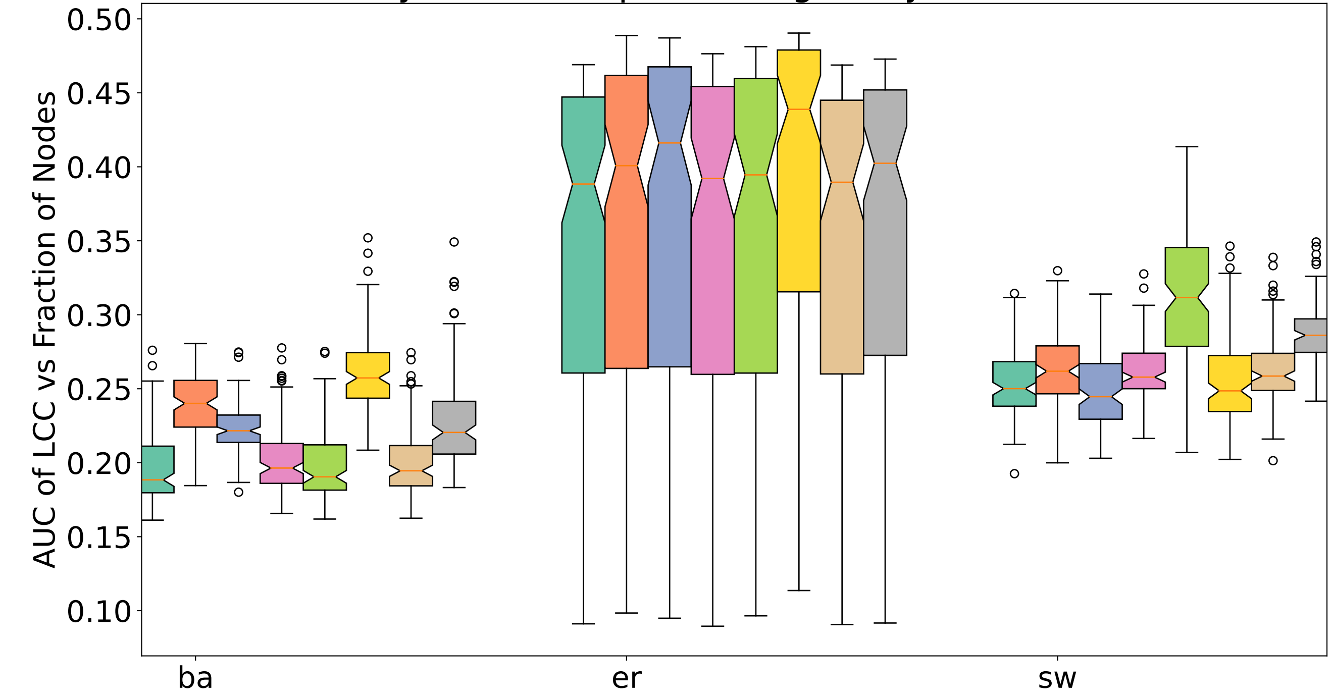
Synthetic Graph: Homogeneity Variation
