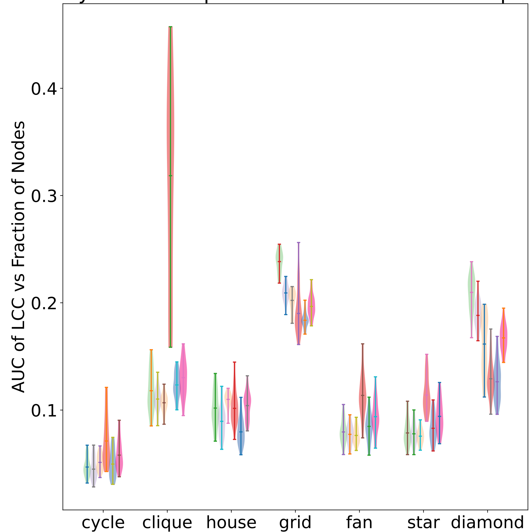
Synthetic Graph with Motifs: Tree Base Graph
