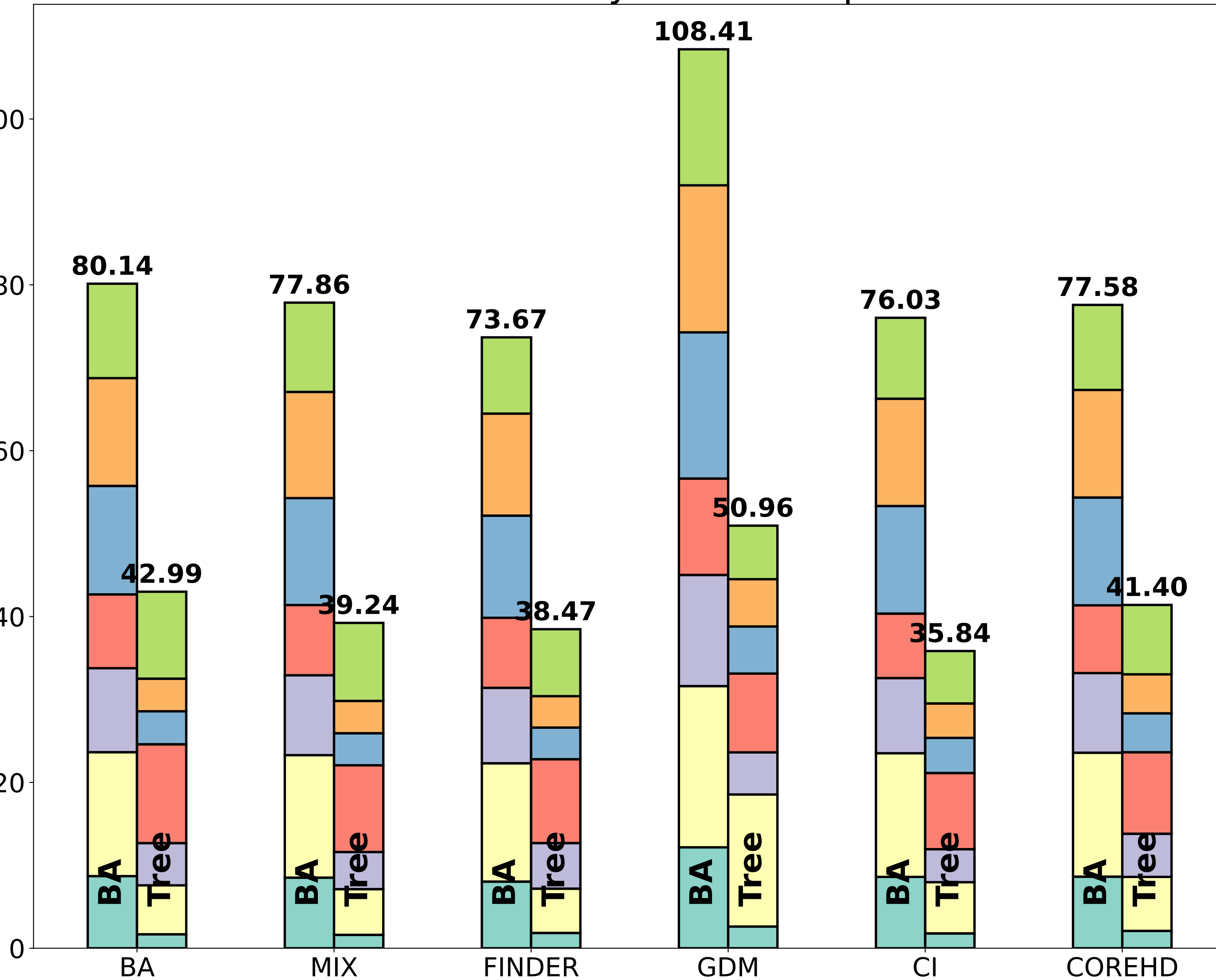
MinMax: Evaluation of models on Synthetic Graph with Motifs Attached
