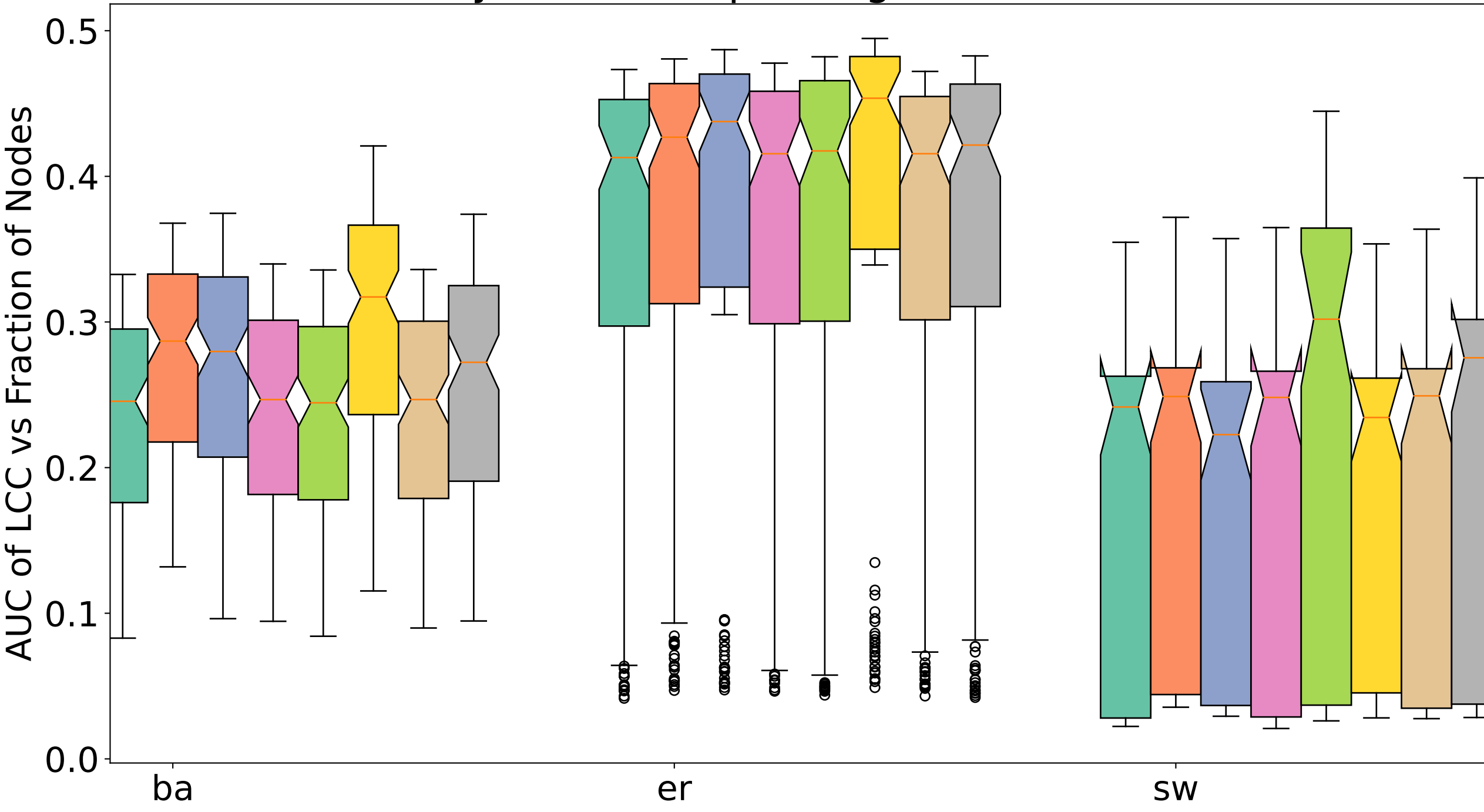
Synthetic Graph: Degree Variation
