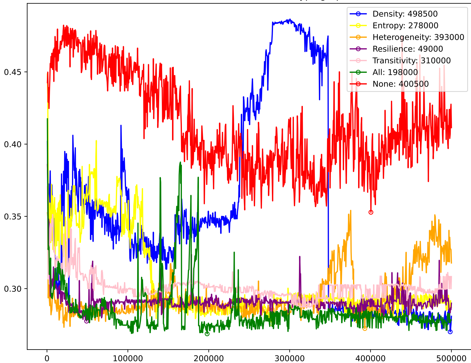
AUC of LCC vs Nodes Plot ALL type graph
