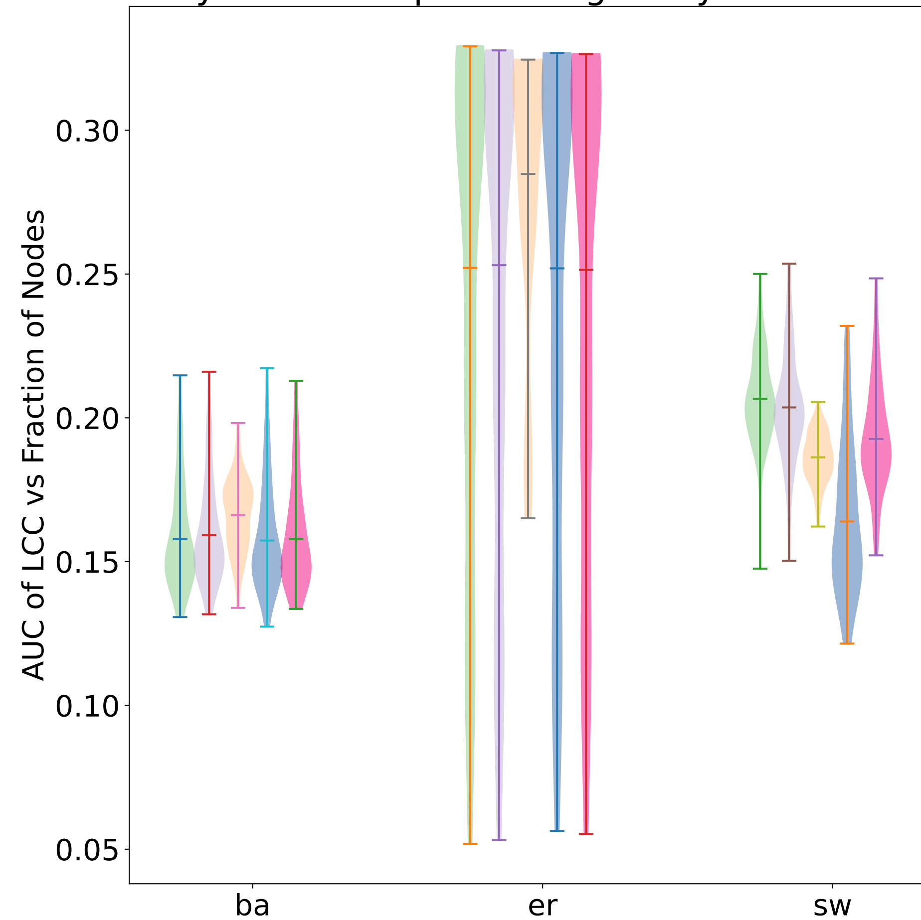
Synthetic Graph: Homogeneity Variation
