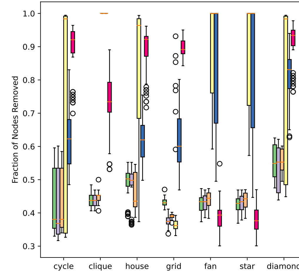
Synthetic Graph with Motifs: Tree Base Graph
