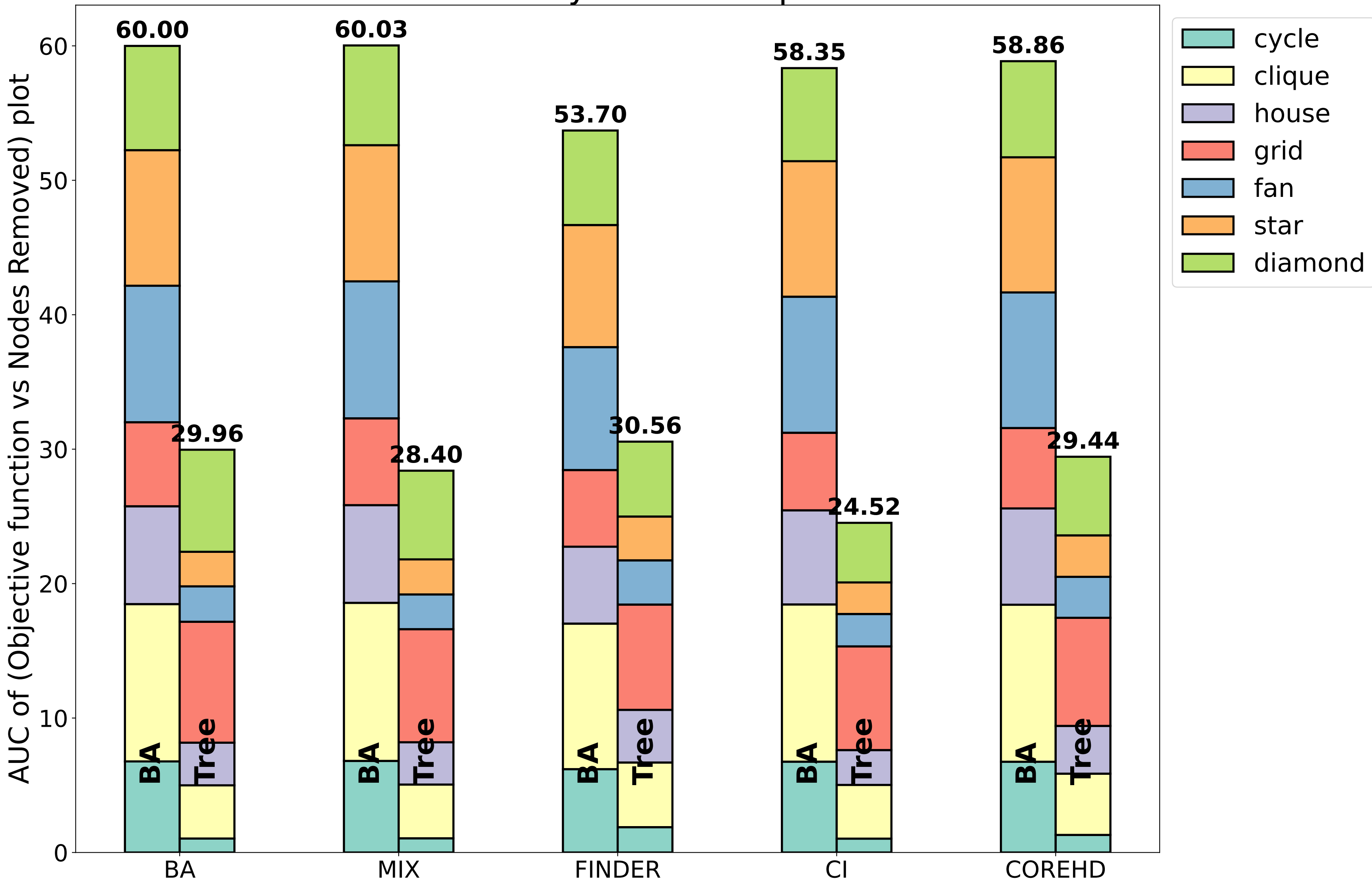
CNP: Evaluation of models on Synthetic Graph with Motifs Attached
