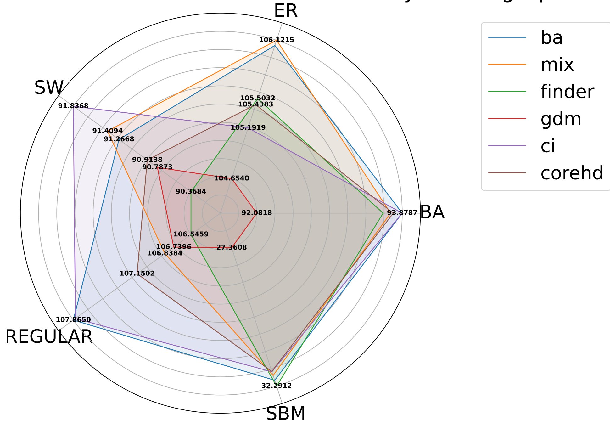
Radar Chart of Cummmulative AUC for different synthetic graph
