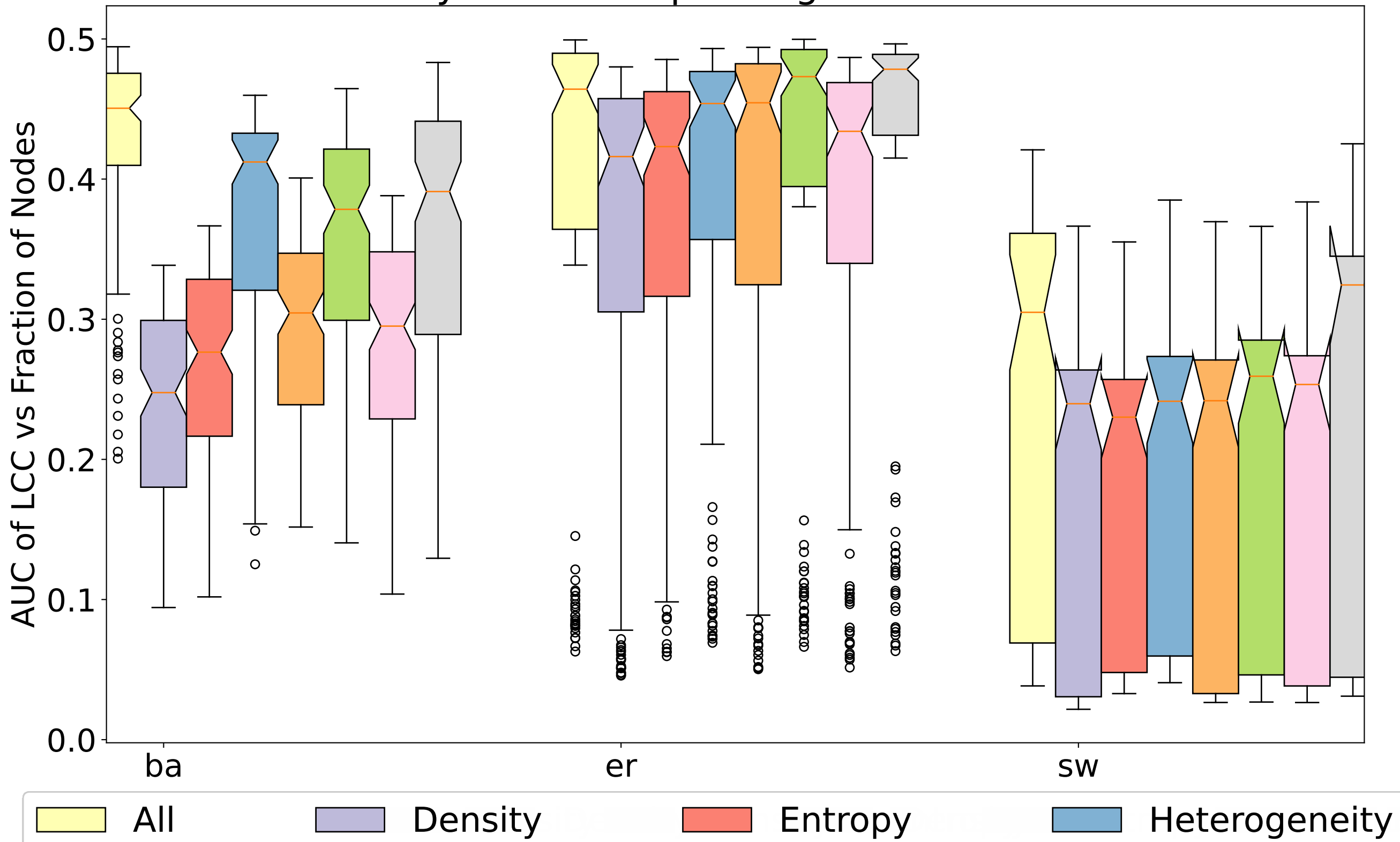
Synthetic Graph: Degree Variation
