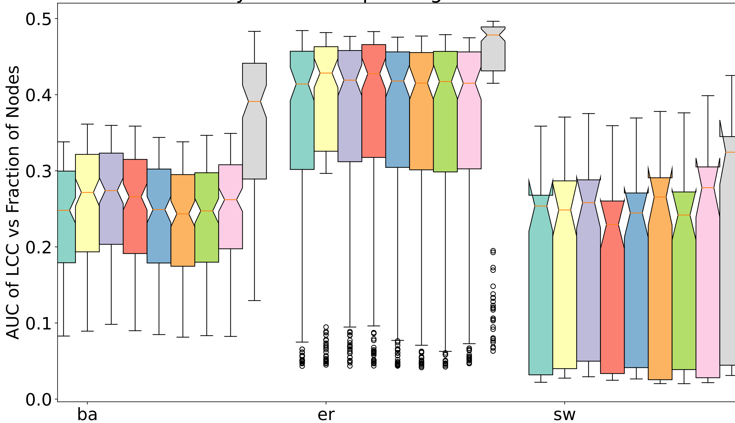
Synthetic Graph: Degree Variation
