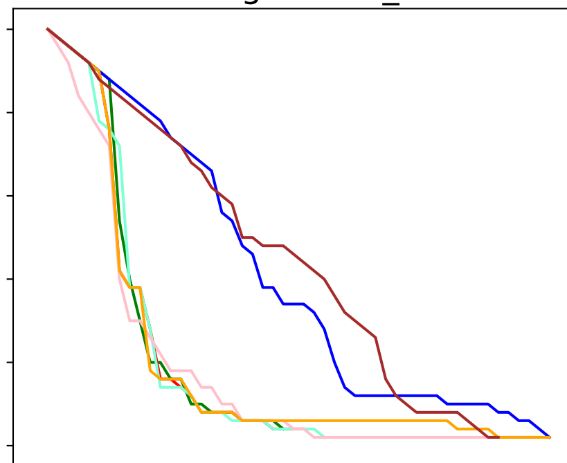
homogeneous_50
