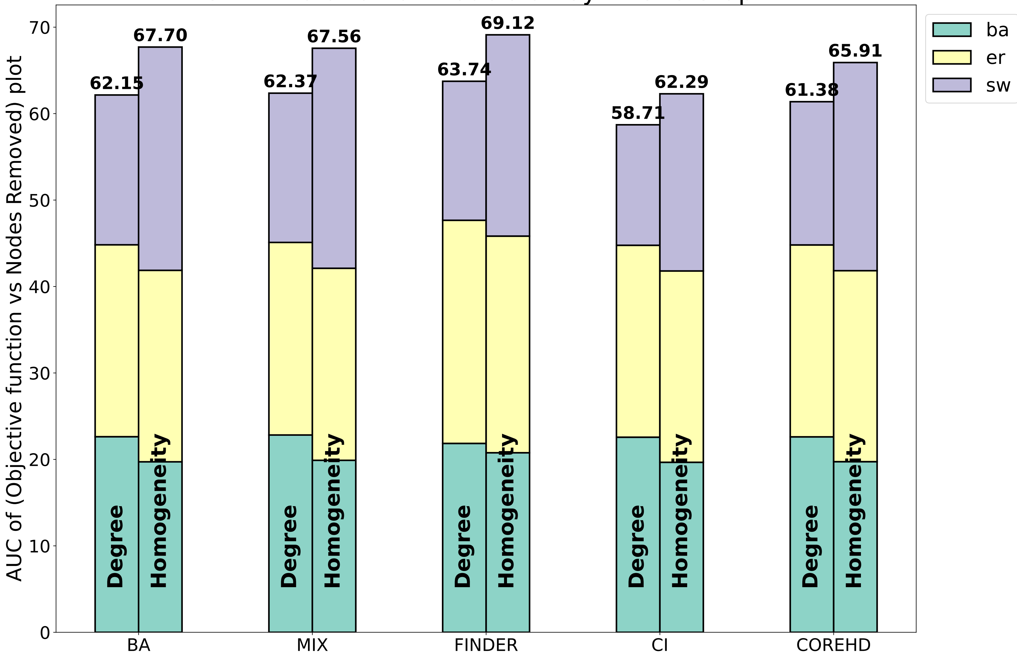
CNP: Evaluation of models on Synthetic Graph
