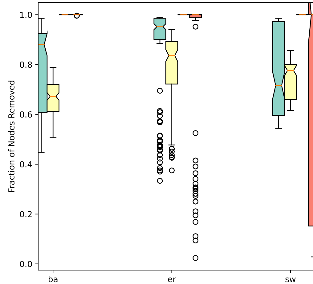
Synthetic Graph: Degree Variation
