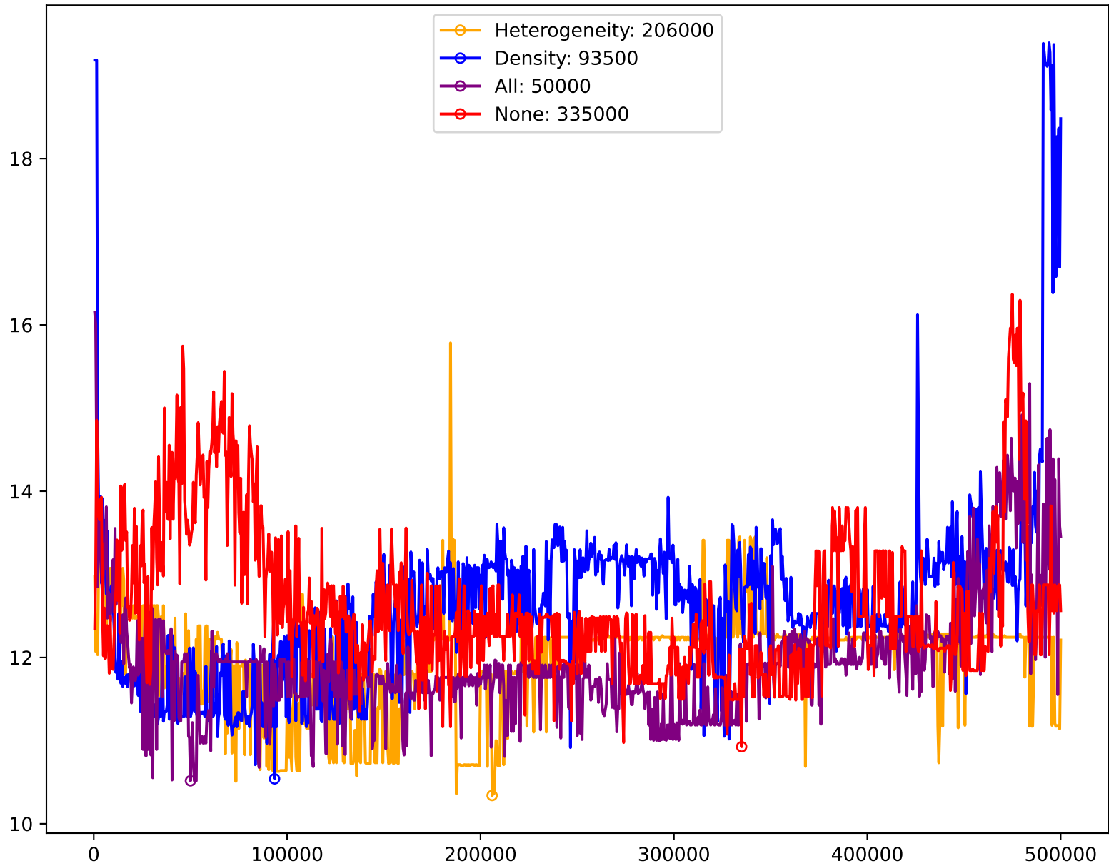
AUC of LCC vs Nodes Plot SW type graph
