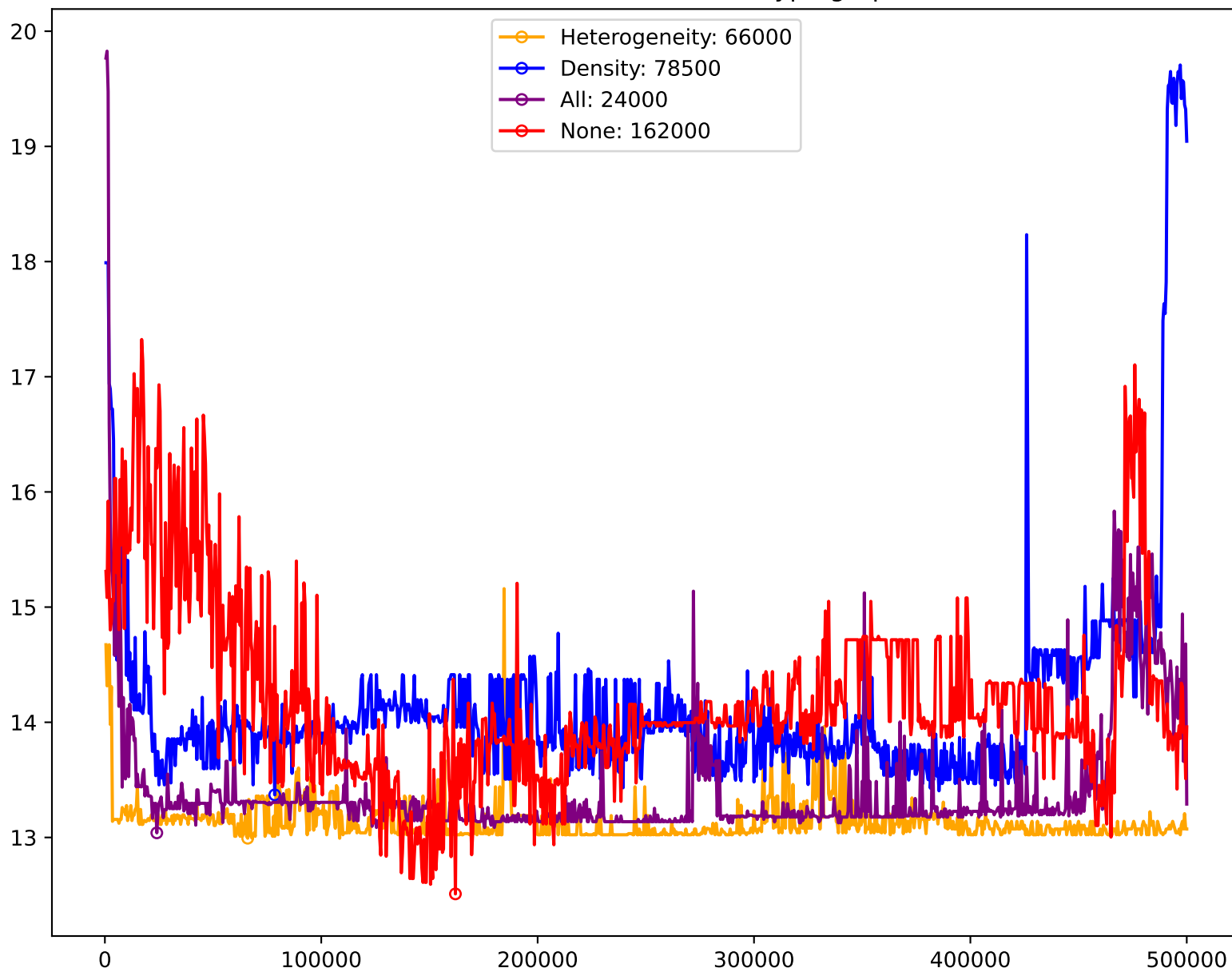
AUC of LCC vs Nodes Plot ER type graph
