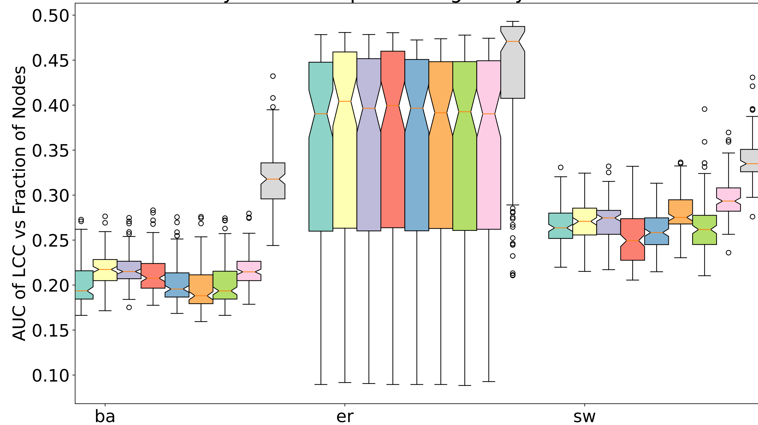
Synthetic Graph: Homogeneity Variation
