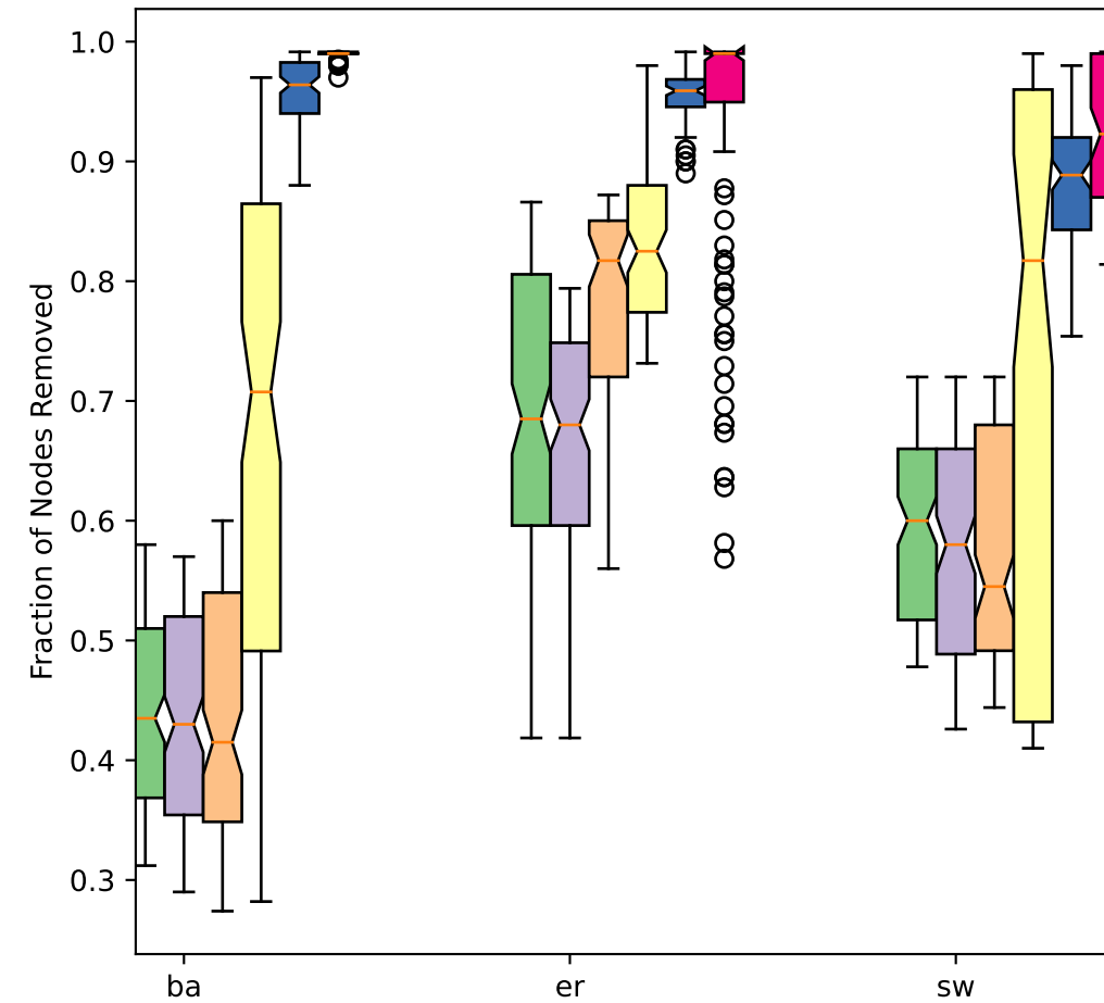
Synthetic Graph: Homogeneity Variation
