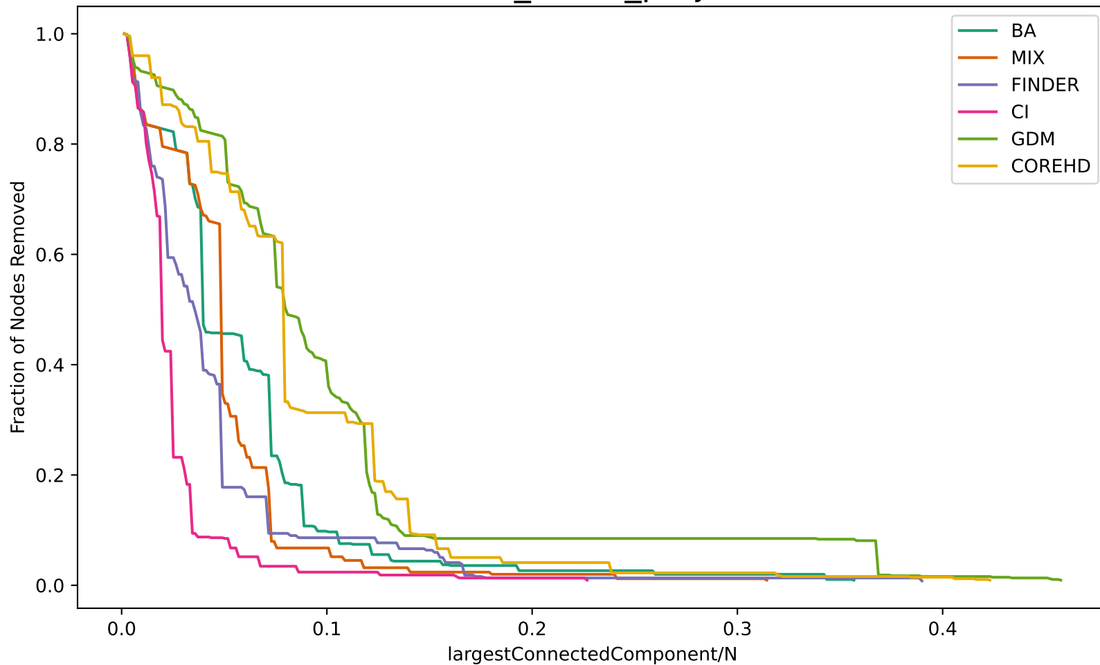
moreno_crime_projected
