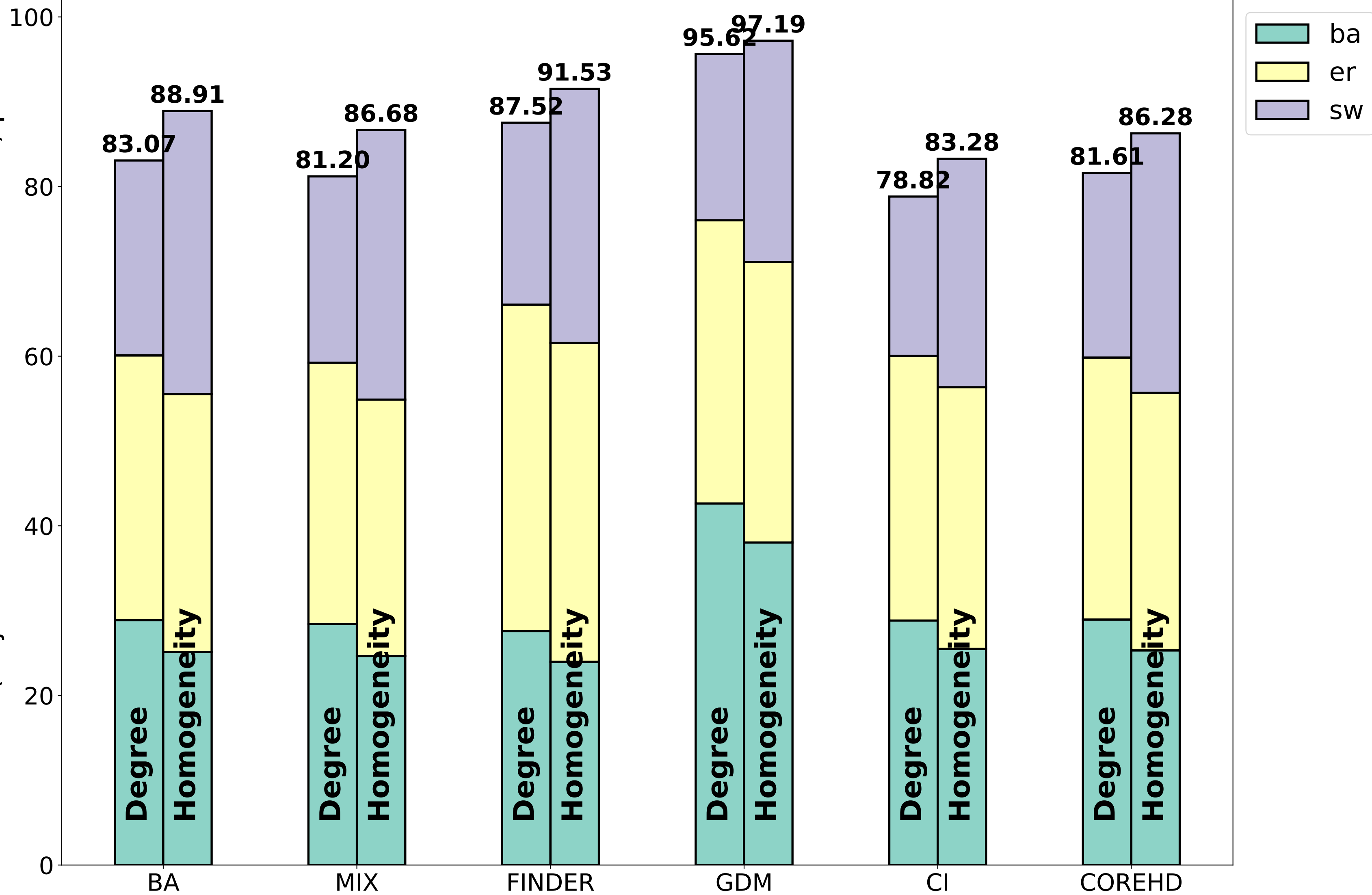
MinMax: Evaluation of models on Synthetic Graph
