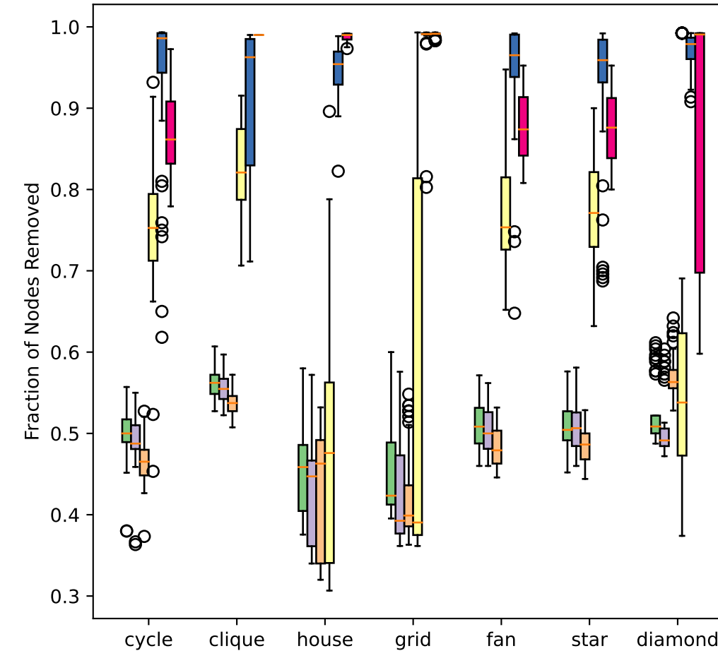
Synthetic Graph with Motifs: BA Base Graph
