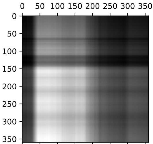
Outer Product
