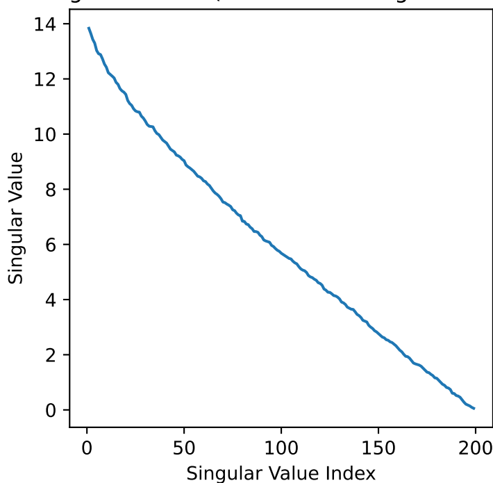
Singular Values (without first singular value)
