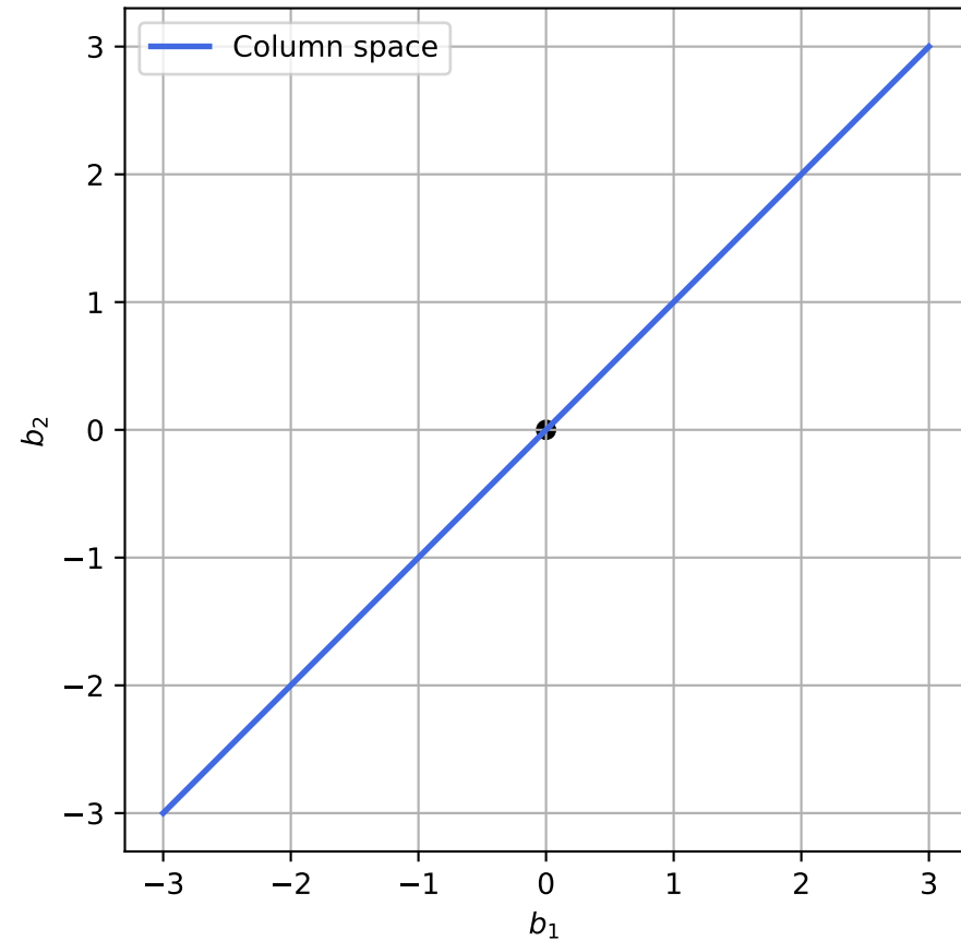
Column space in \mathbb{R}^2
